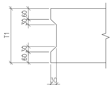
SHEAR KEY DETAIL
