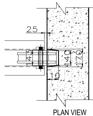
JACKING & SUPPORT BEAM TILTFOOT SET OUT DETAIL
