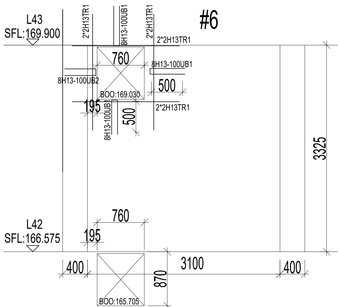
WINDOW RECESS HOR-BAR
