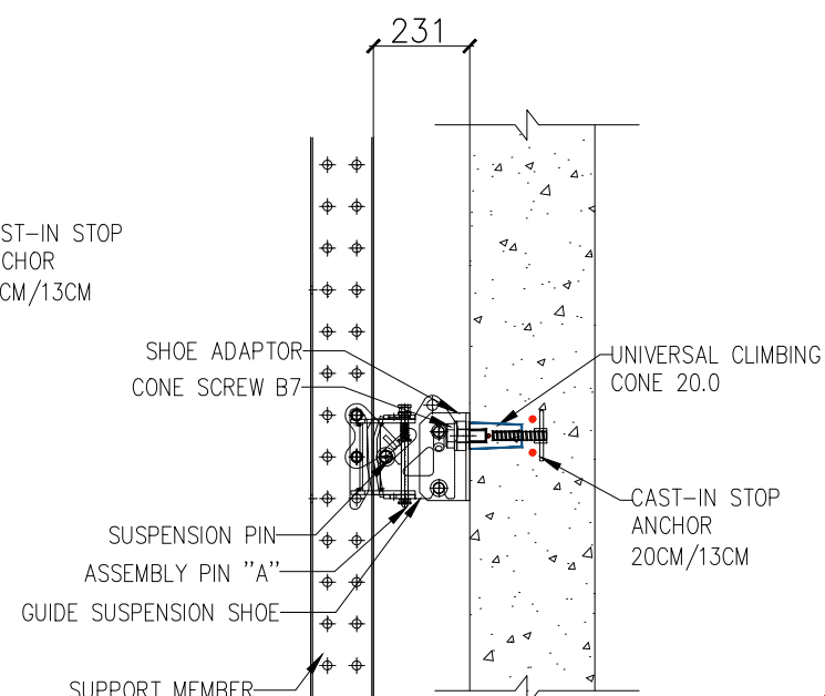
SIDE VIEW - ANCHOR DETAIL FOR GUIDE SUSPENSION SHOE
