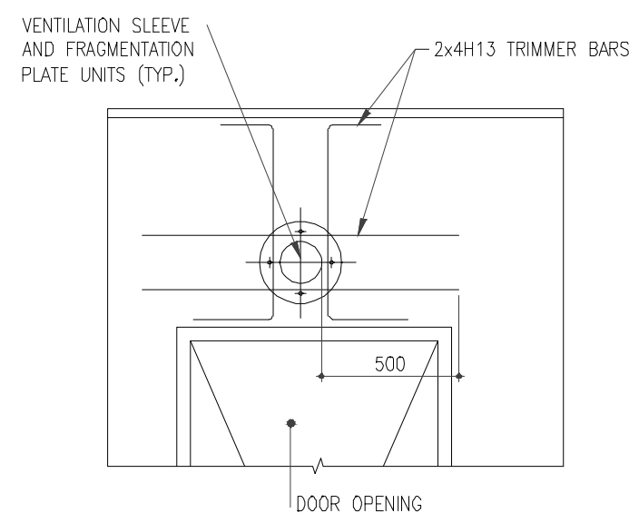
TYPICAL DETAIL OF TRIMMER BARS FOR VENTILATION SLEEVE
