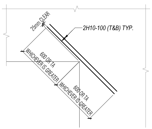
TYPICAL TRIMMER BARS AT RE-ENTRANT CORNER SCALE : 1:25
