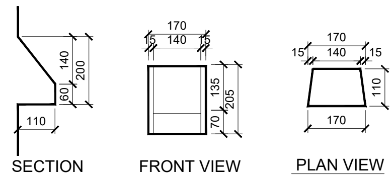
DETAIL-1: Required wall Recess Dimensions for Tiltfoot Pockets of Jacking & Support Beam for Auto climb wallform system
