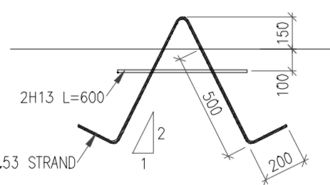
LIFTING HOOK DETAIL
