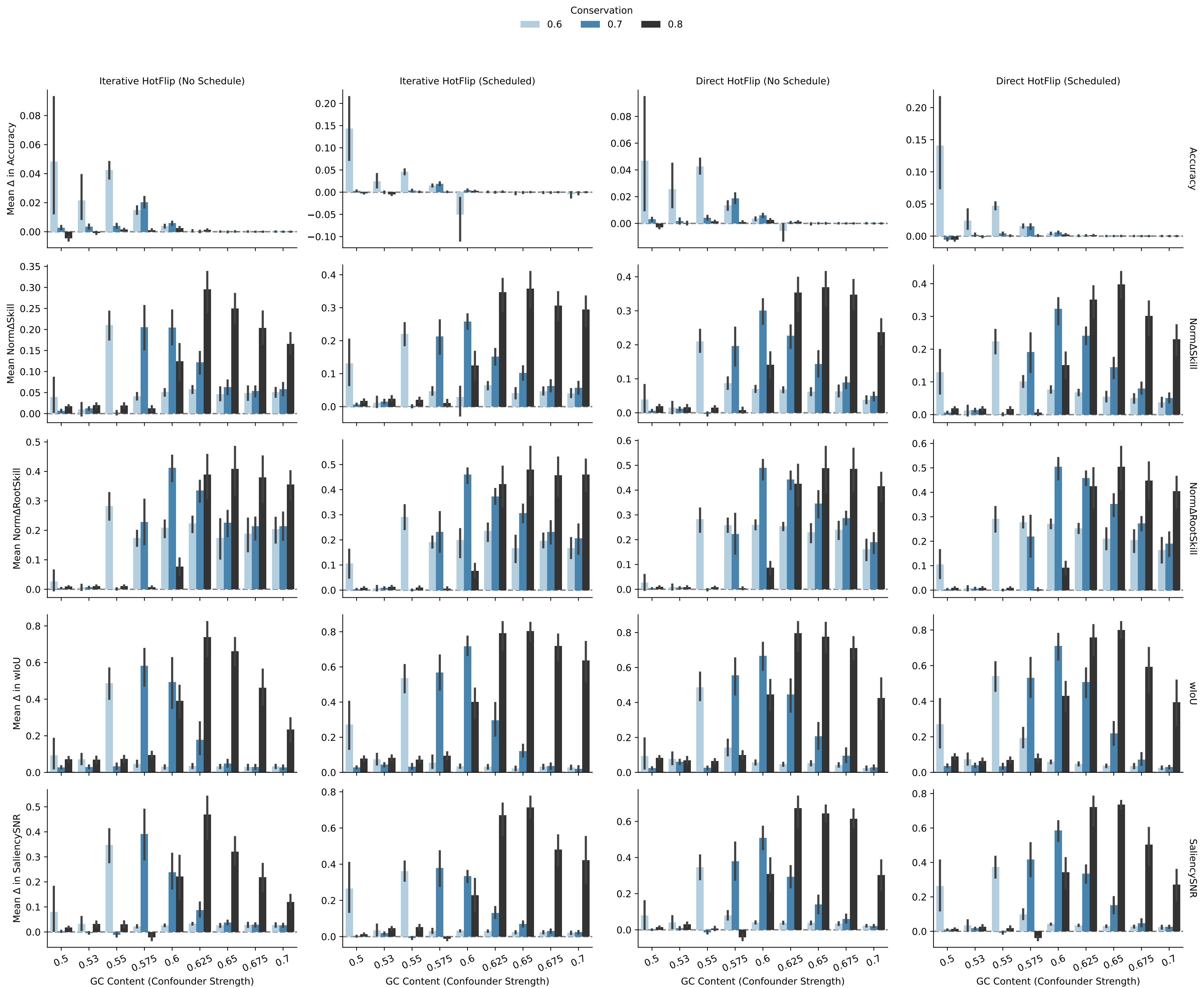
Comparison of Training Strategies: Mean Improvement vs. Standard Model (Best \varepsilon selected by \Delta RootSkill; error bars show SE across 10 seeds)
