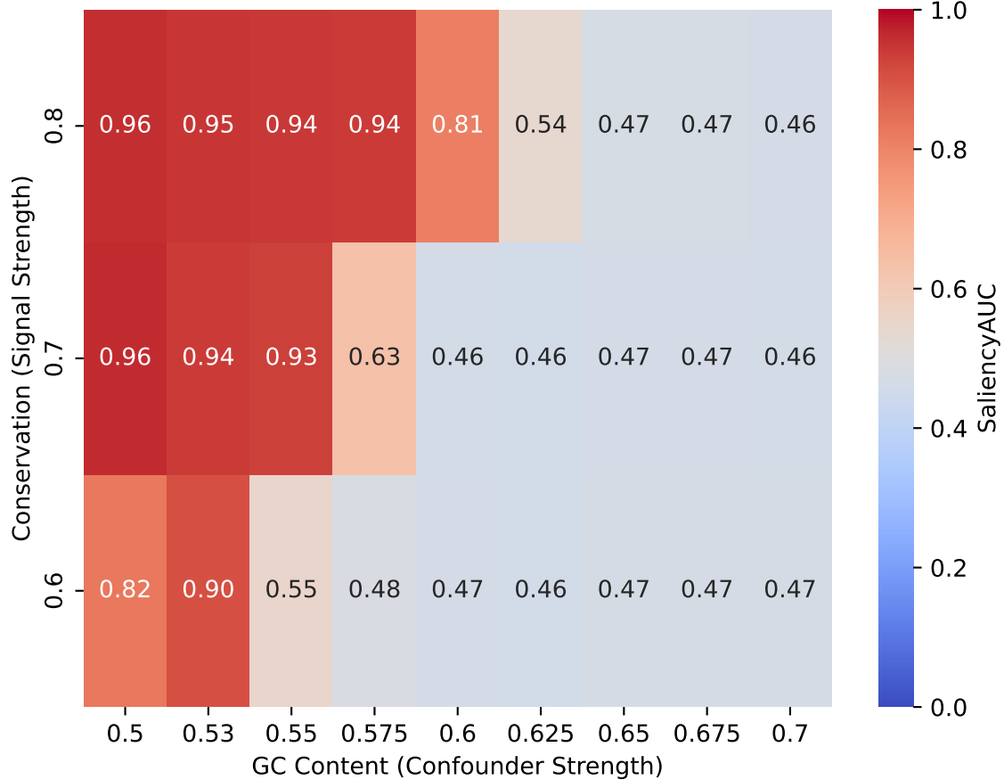
Standard Model
