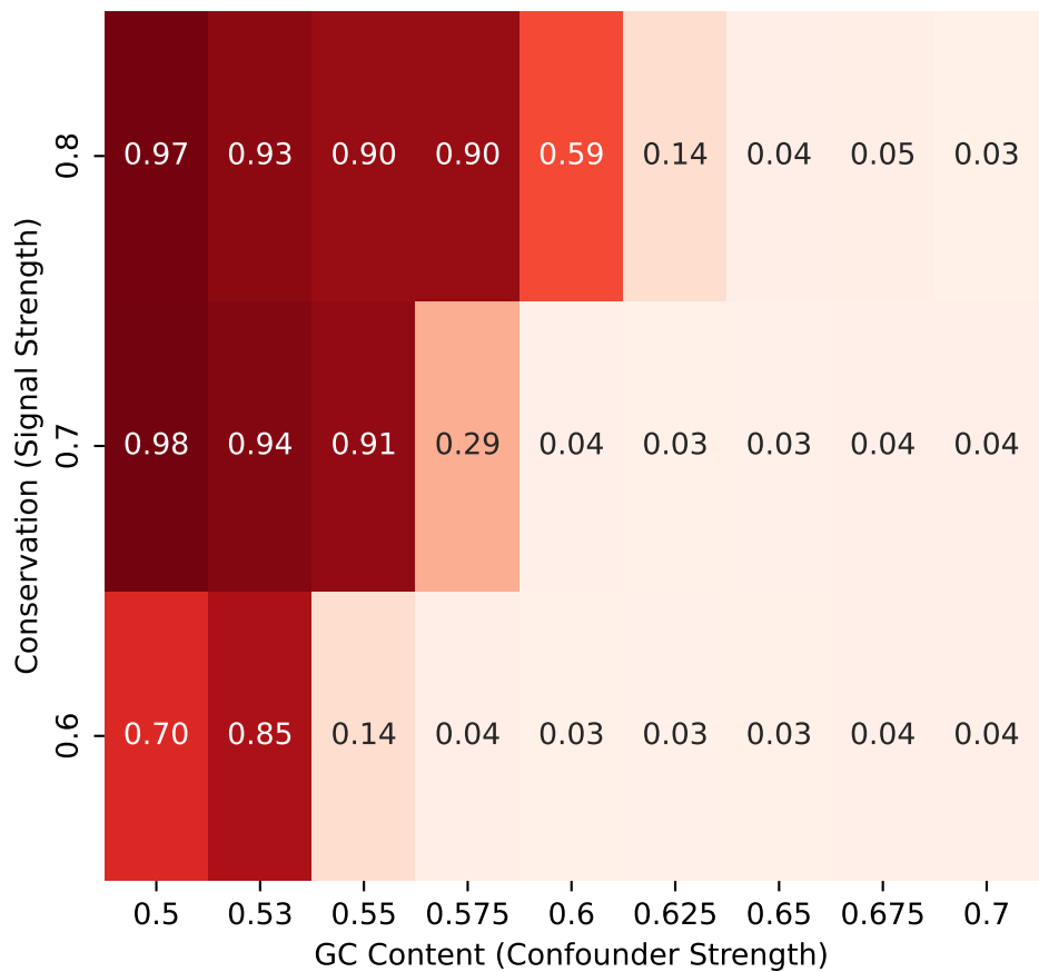
Standard Model
