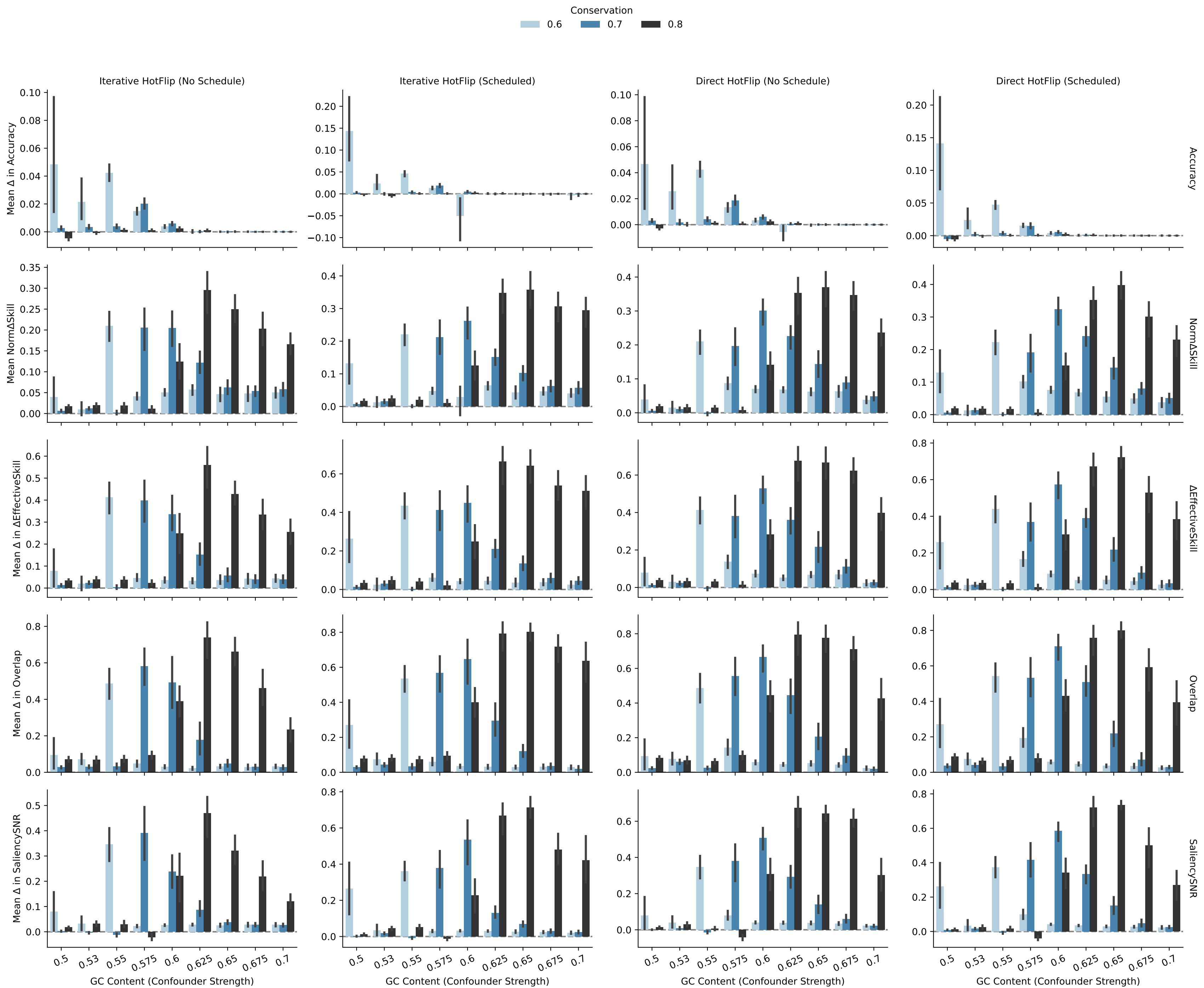
Comparison of Training Strategies: Mean Improvement vs. Standard Model (Best \epsilon selected by \Delta\text{EffectiveSkill} ; error bars show SE across 10 seeds)
