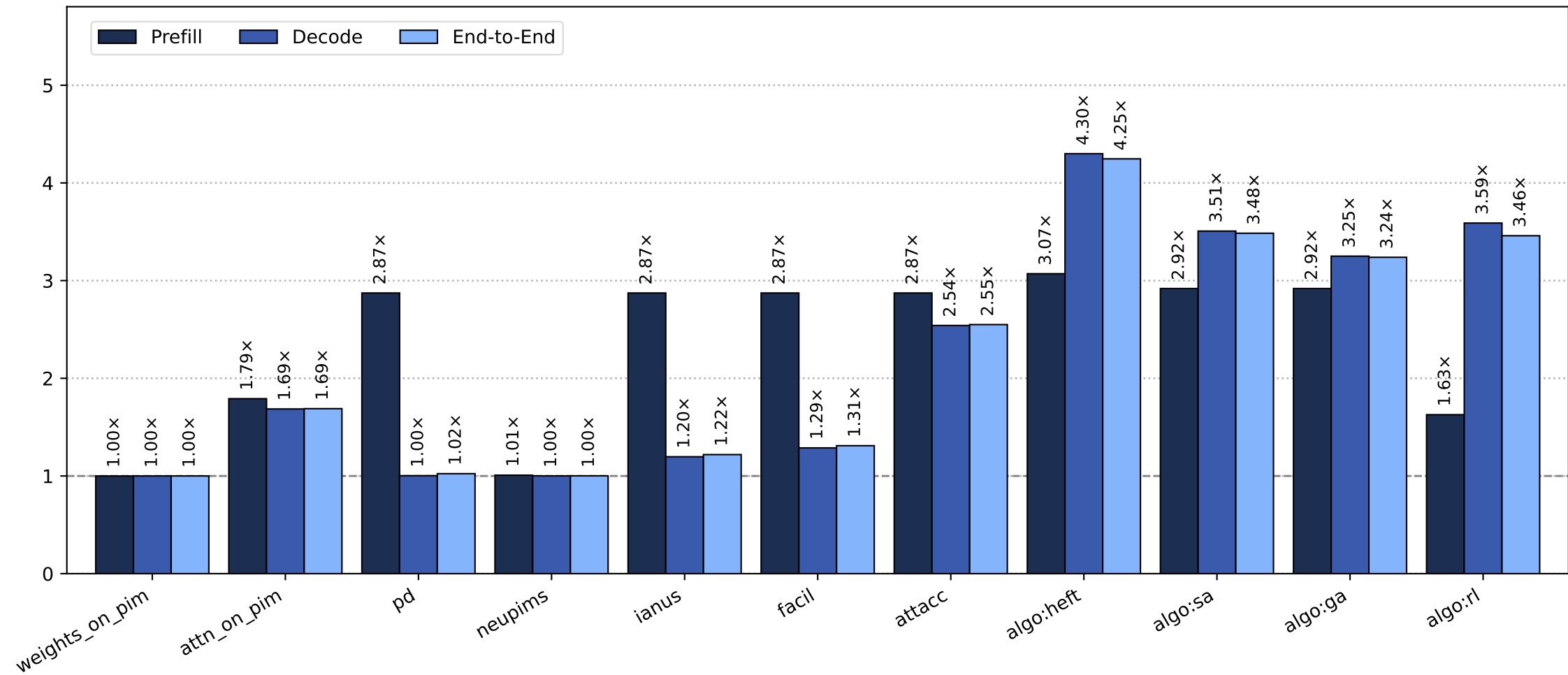
Prefill & Decode Speedup
