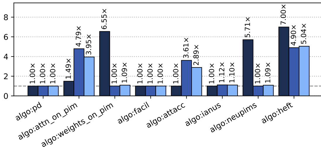
S=128, T=128
