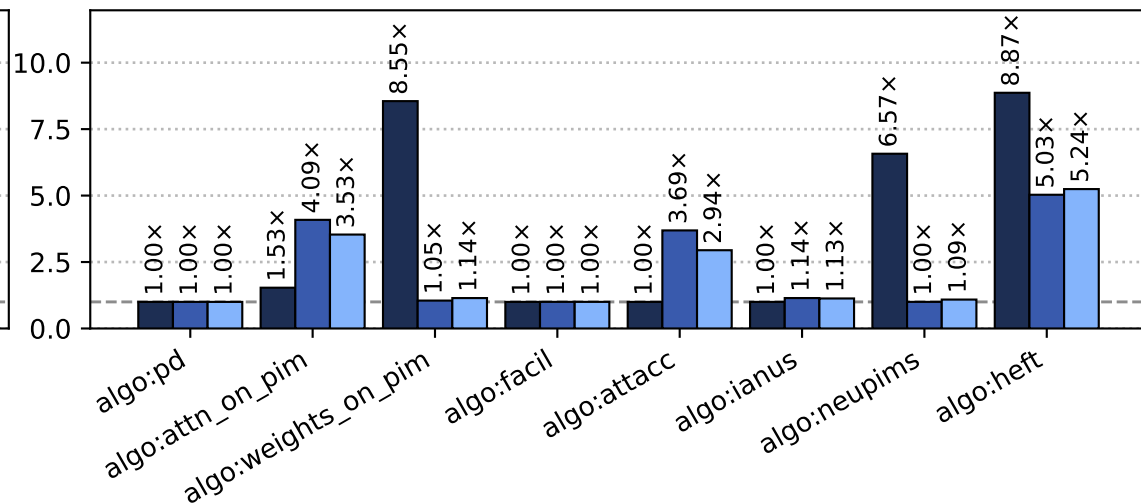
S=1024, T=1024
