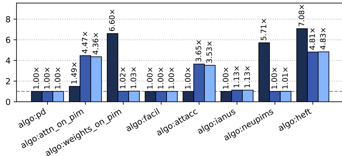
S=128, T=1024
