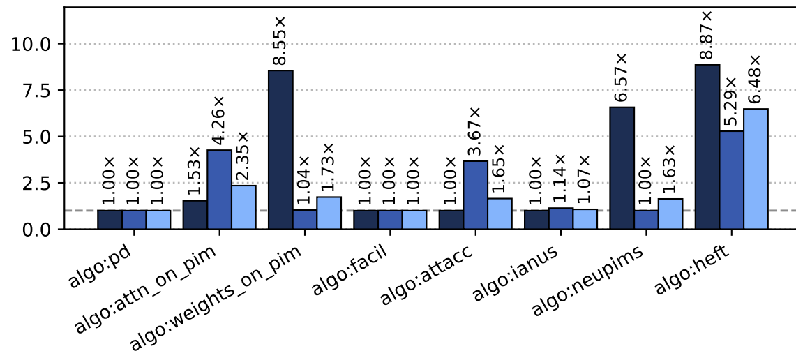
S=1024, T=128
