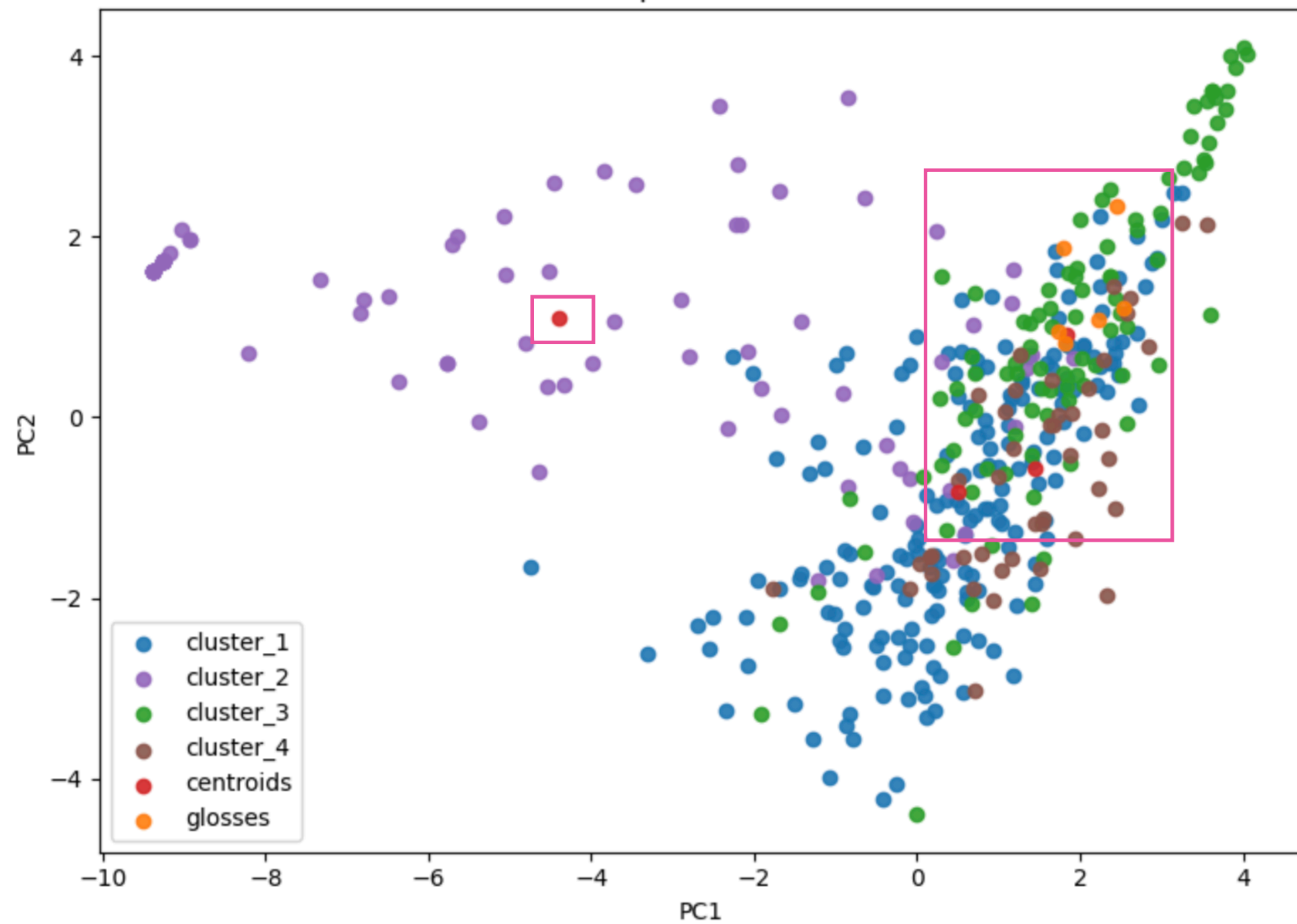
PCA Scatterplot (Trunk, masked)
