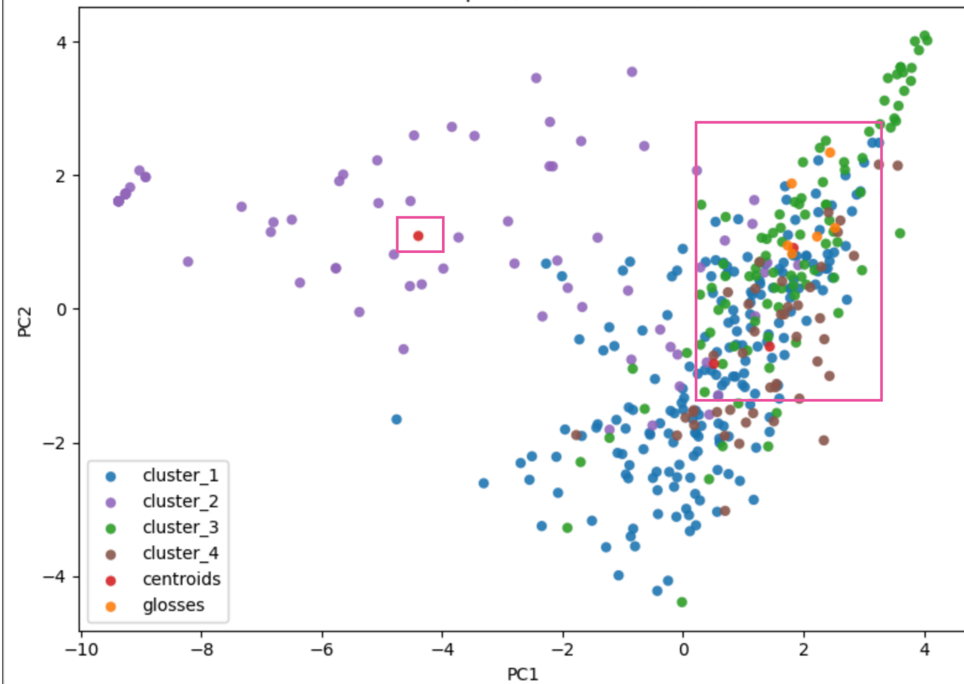
PCA Scatterplot (Trunk, unmasked)
