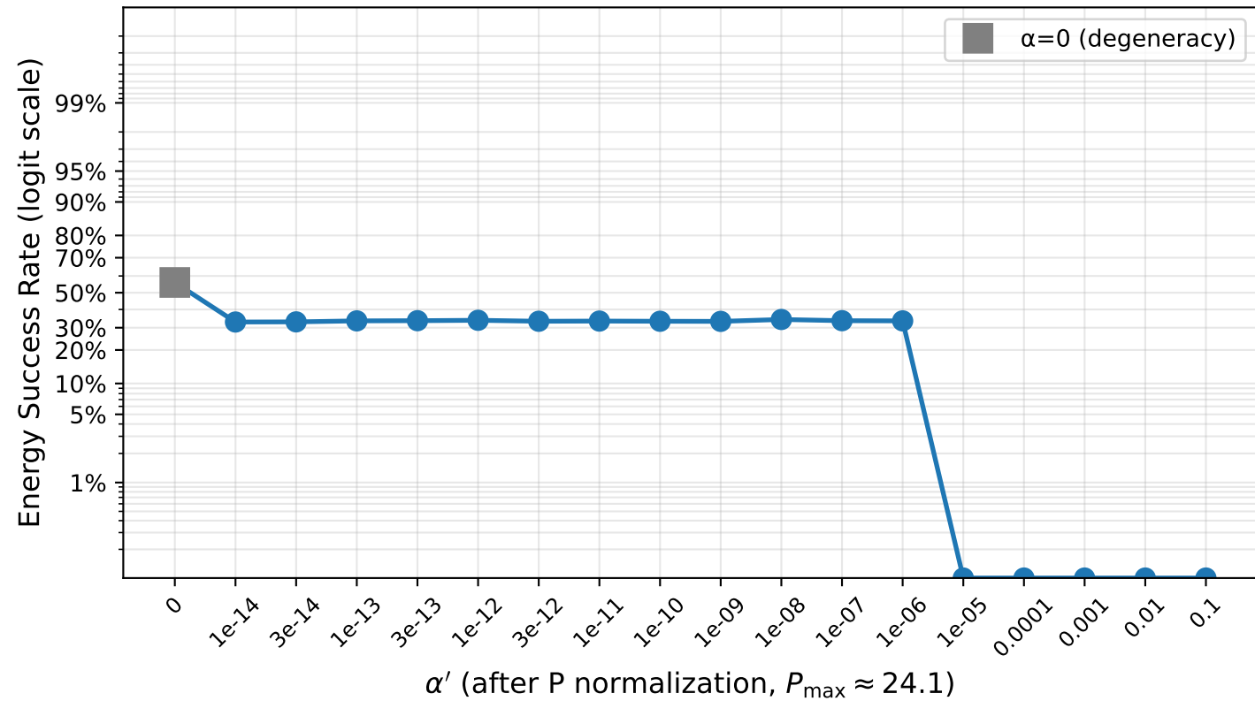
(b) Logit scale — transition region \square\square
