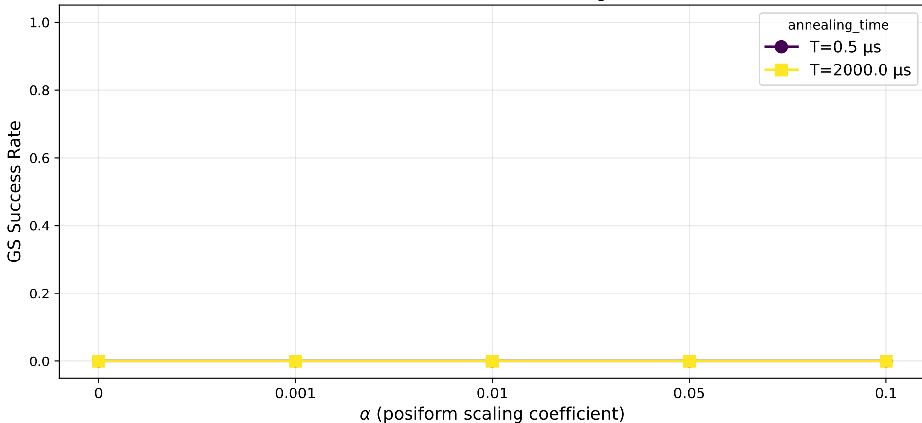
QPU GS GSP vs \alpha \times anneal time — Pegasus P16, lin2
