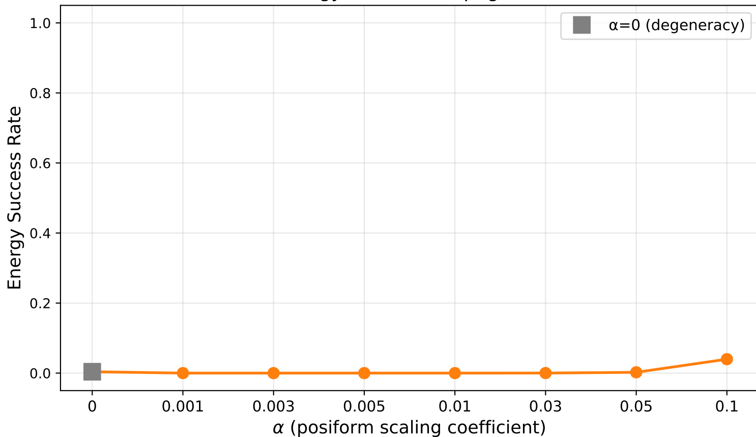
QPU Energy GSP vs \alpha — pegasus, lin2
