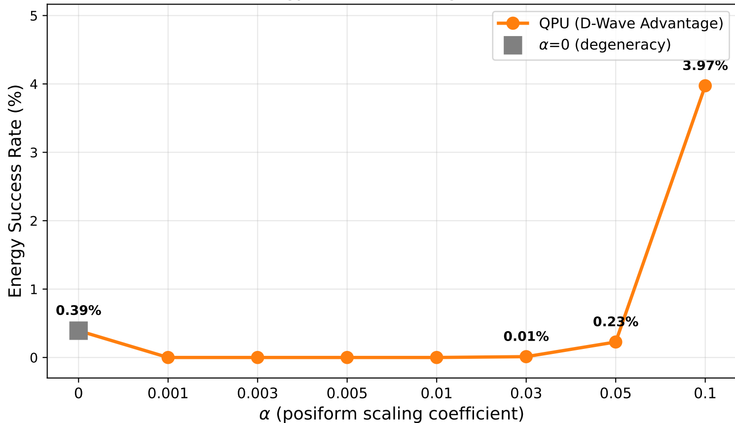
QPU Energy GSP vs \alpha — Pegasus P16, lin2
