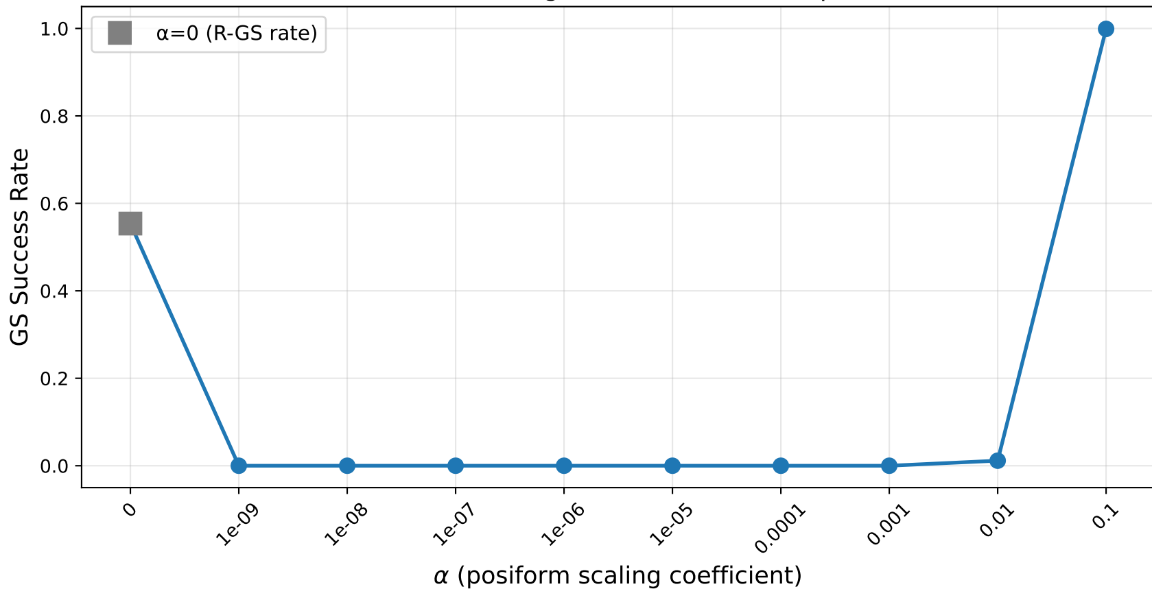
GS GSP vs \alpha — Pegasus P16, lin2, sweep=1000
