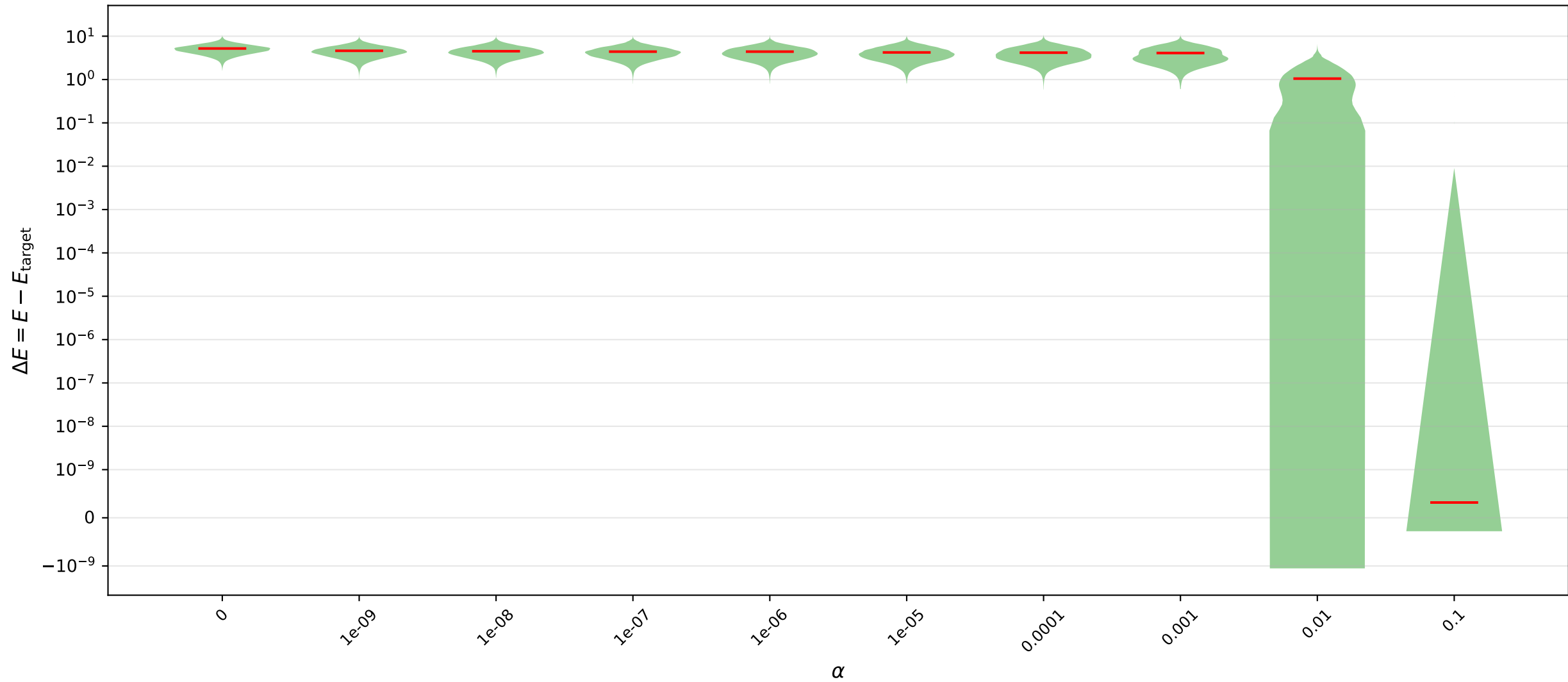
(A) \Delta E distribution per \alpha — Pegasus P16, lin20, sweep=1000, 200 inst \times 100 reads
