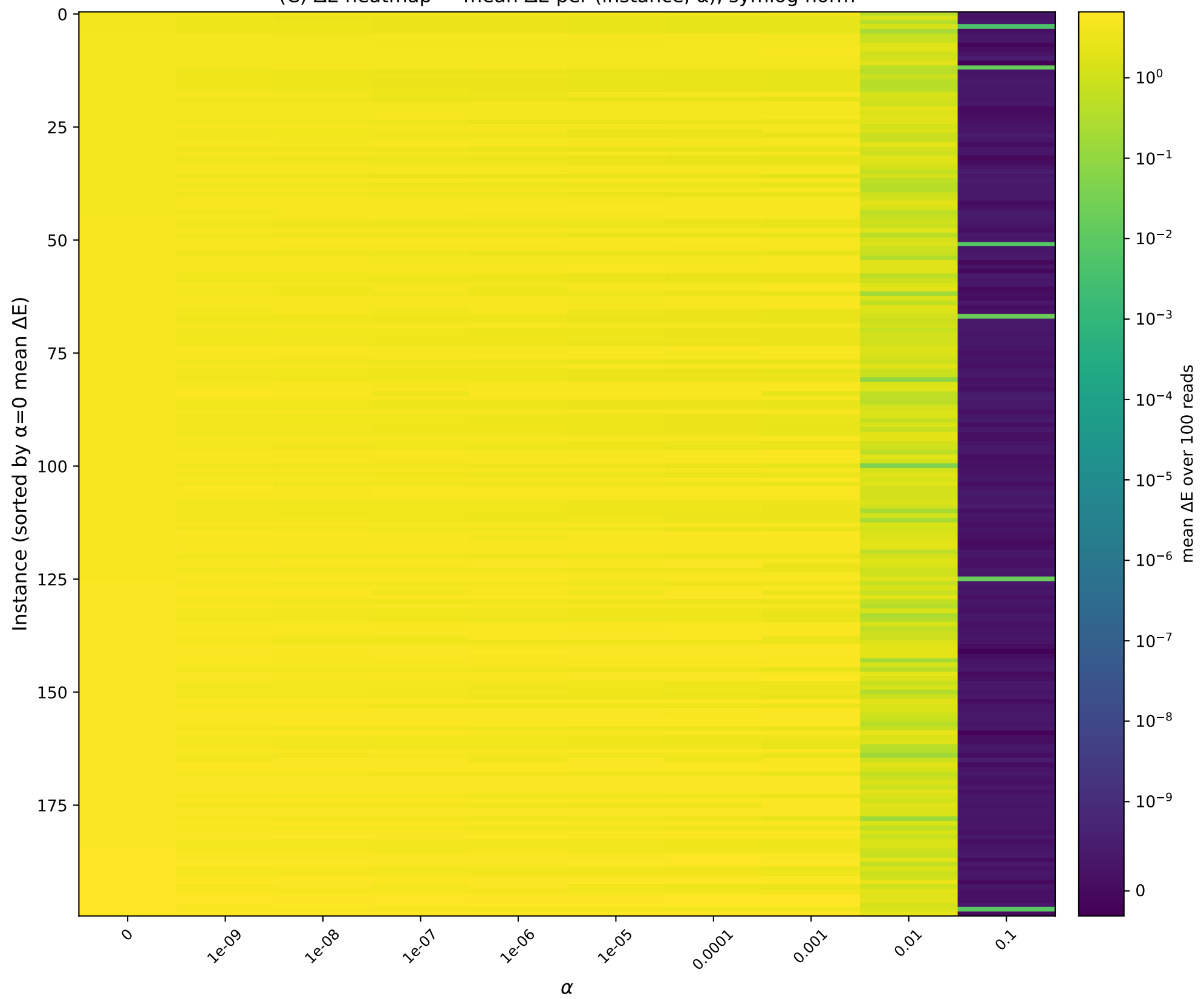
(C) \Delta E heatmap — mean \Delta E per (instance, \alpha ), symlog norm
