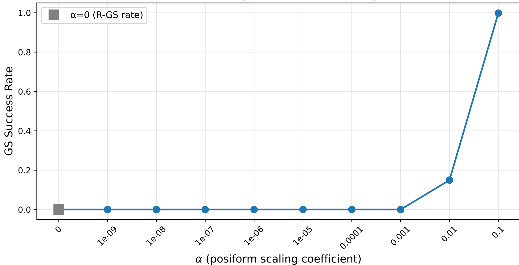
GS GSP vs \alpha — Pegasus P16, lin20, sweep=1000
