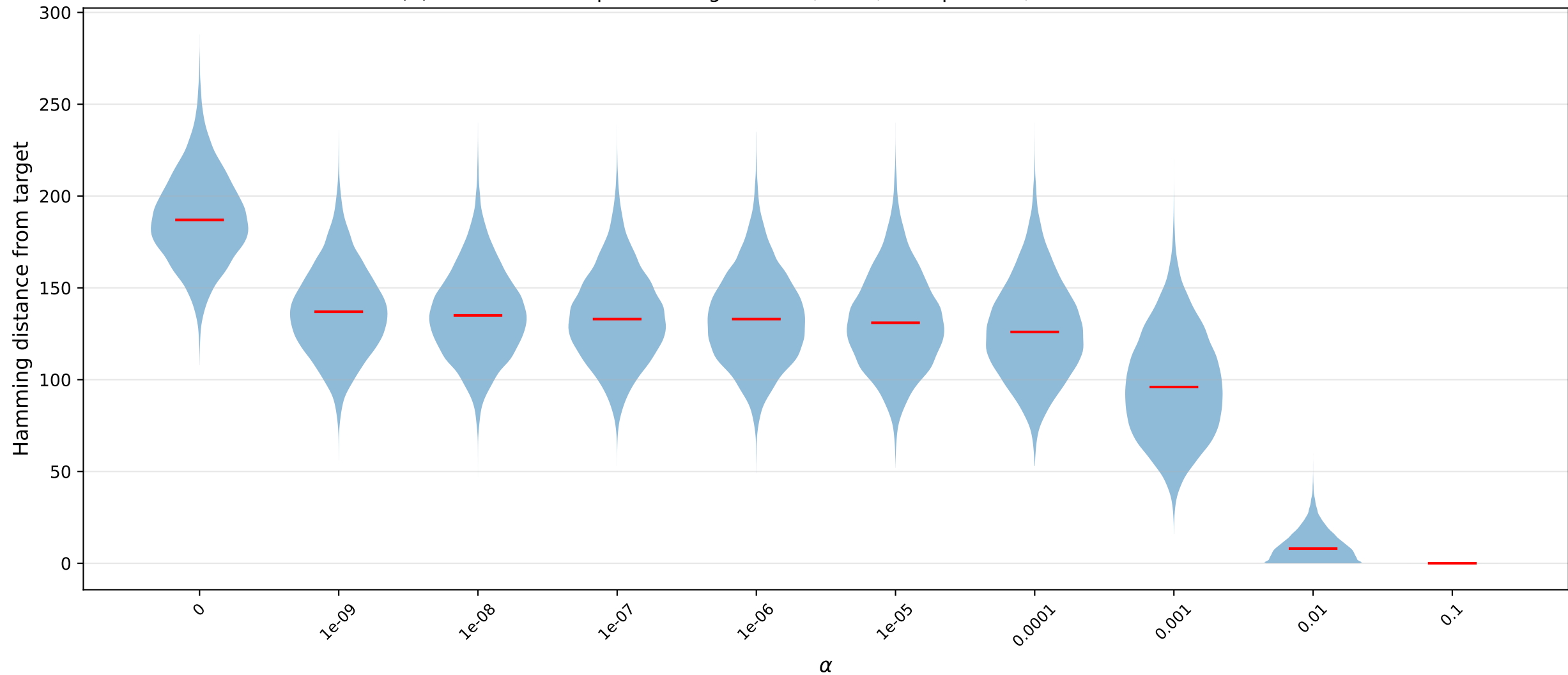
(A) HD distribution per \alpha — Pegasus P16, lin20, sweep=1000, 200 inst \times 100 reads
