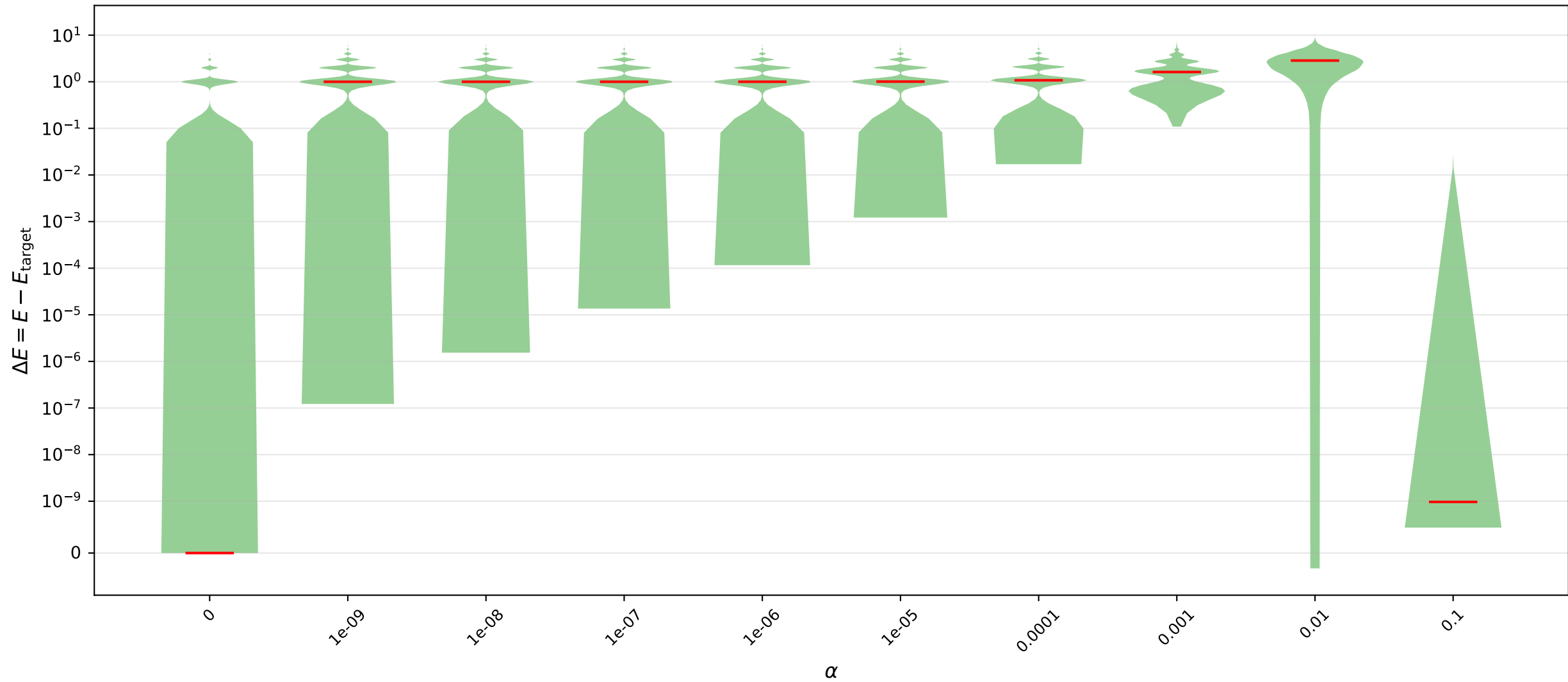
(A) \Delta E distribution per \alpha — Pegasus P16, lin2, sweep=1000, 200 inst \times 100 reads
