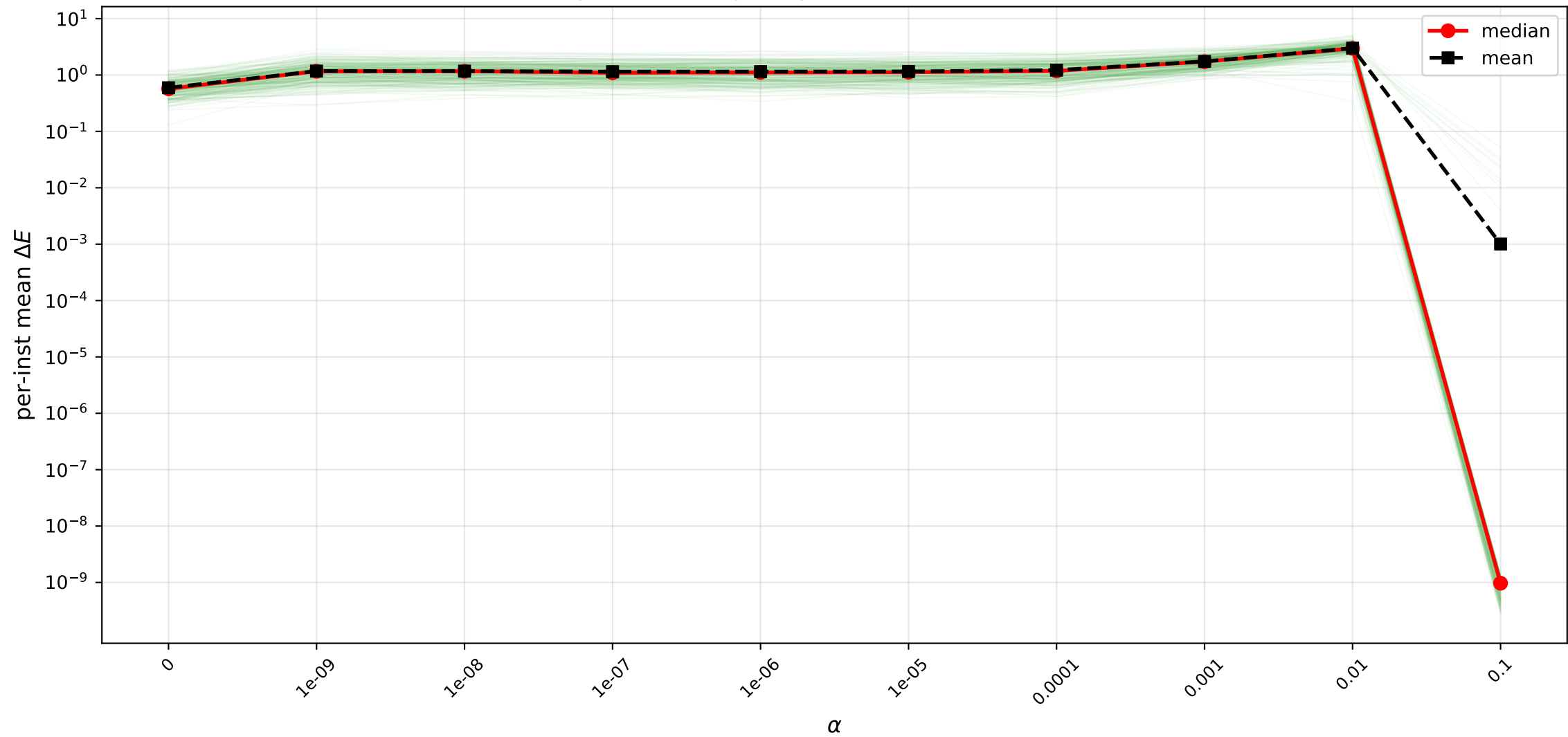
(D) per-inst \Delta E trajectory across \alpha (faded = each inst)
