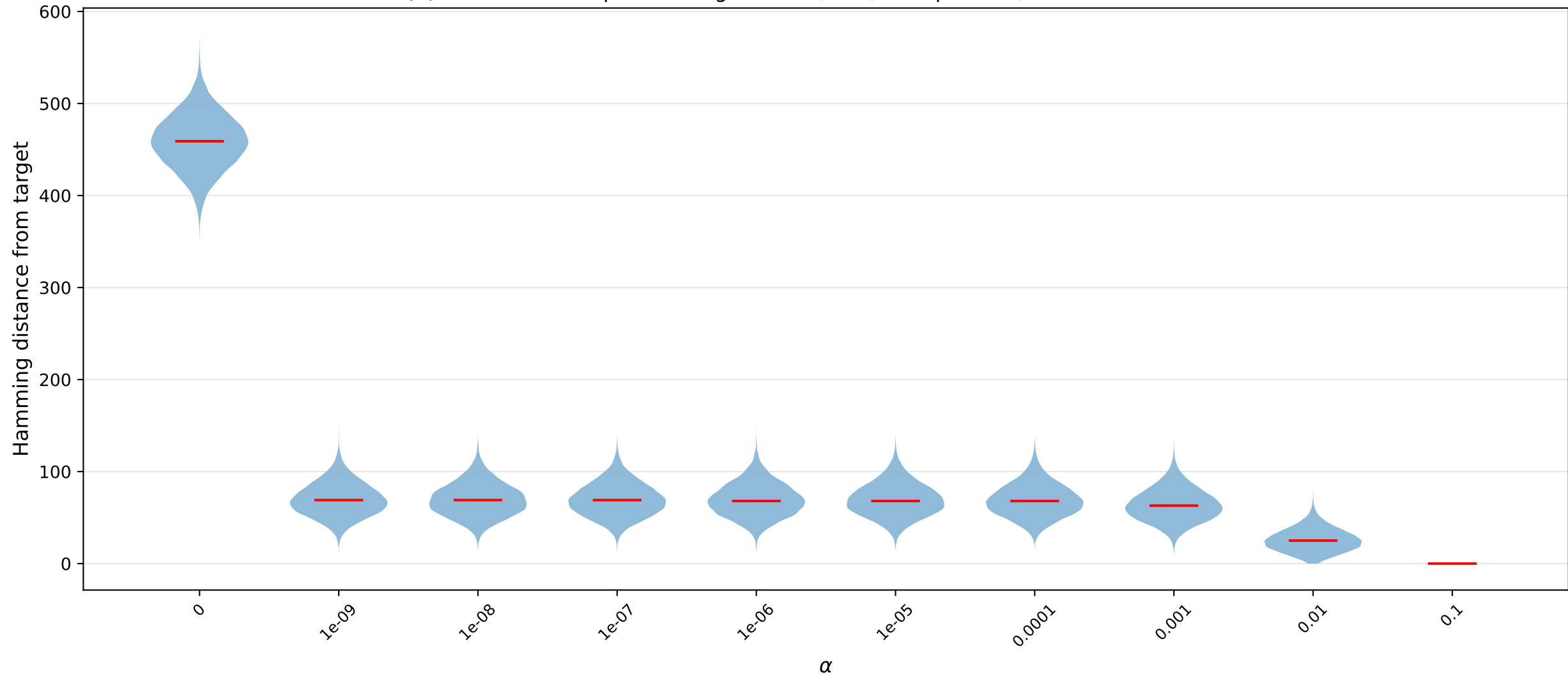
(A) HD distribution per \alpha — Pegasus P16, lin2, sweep=1000, 200 inst \times 100 reads
