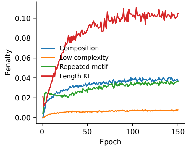
Regularization
