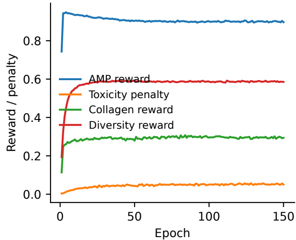
Generator Objectives
