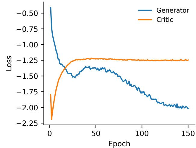
WGAN-GP Loss
