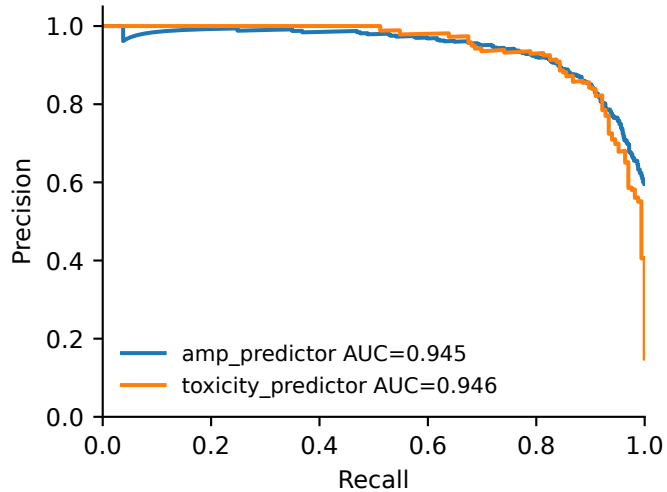
Precision-Recall Curve
