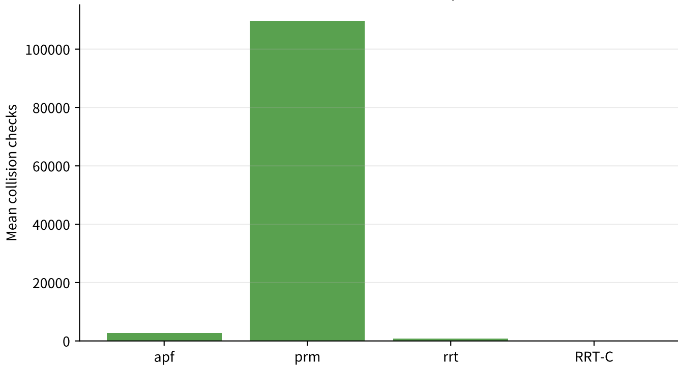
Collision-check count comparison
