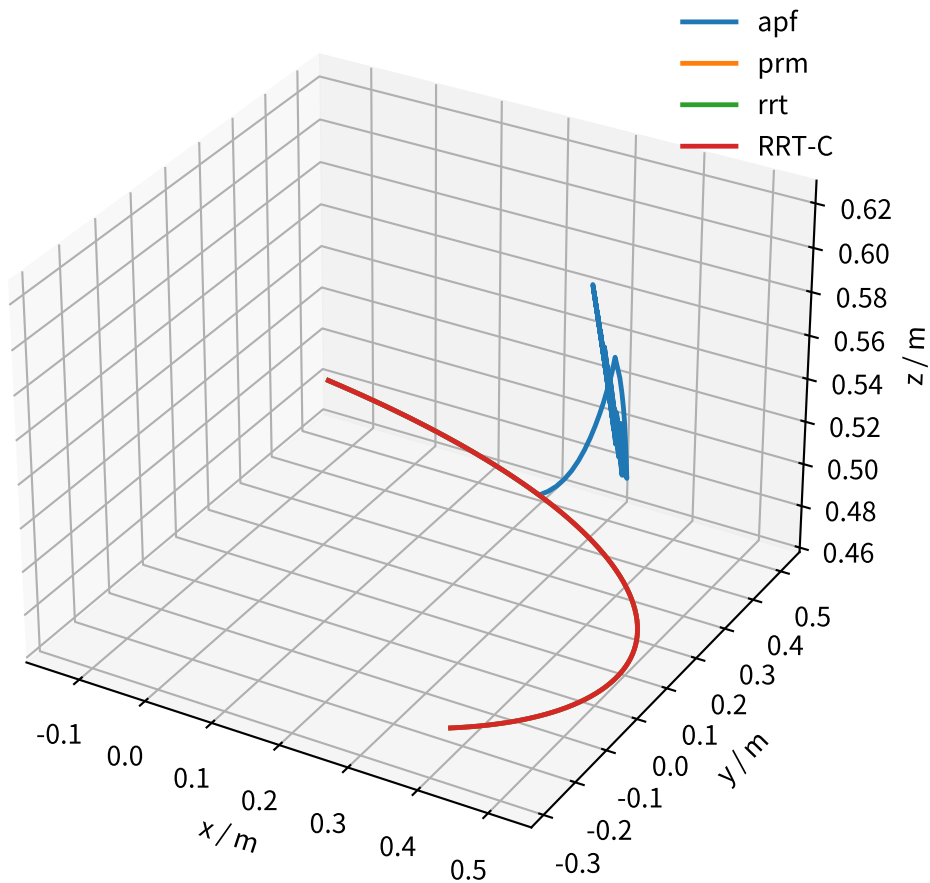
End-effector trajectory: scene_02_multi_obstacles
