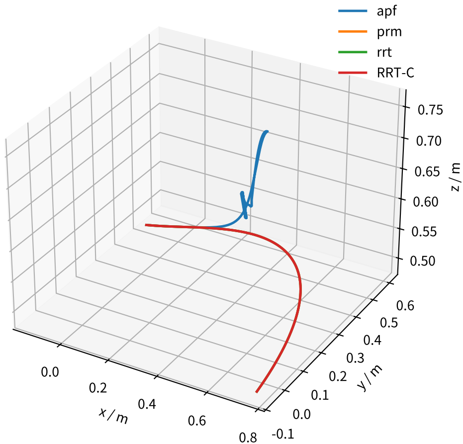
End-effector trajectory: scene_04_near_singularity
