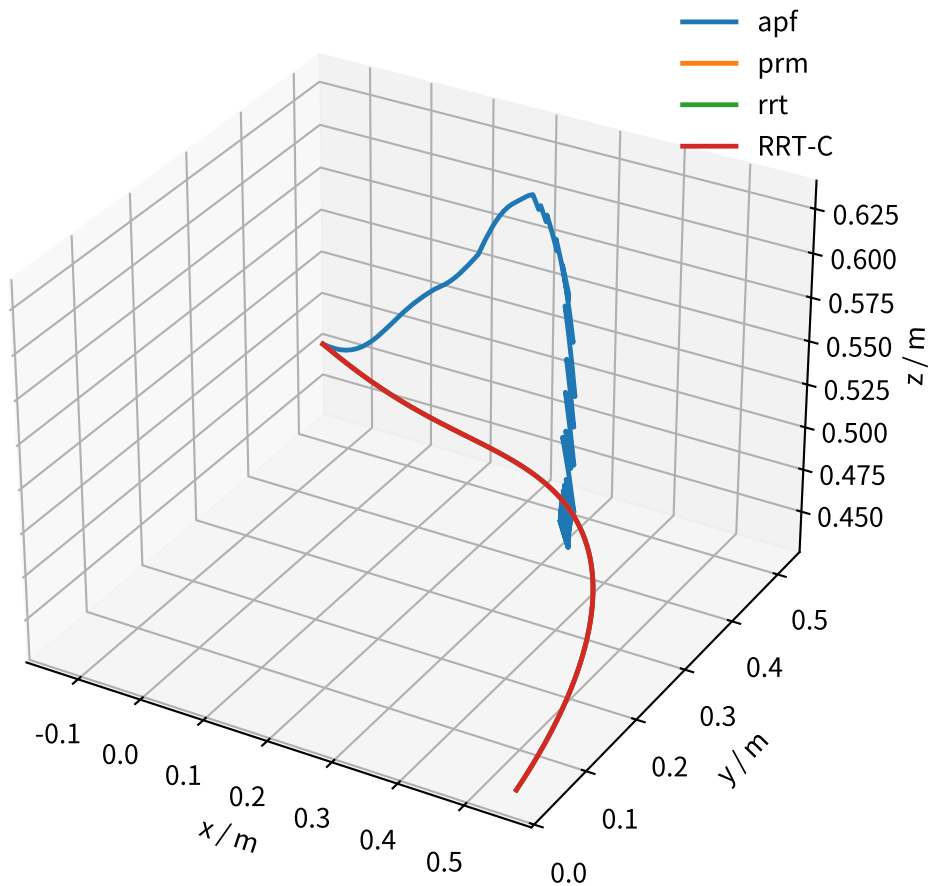
End-effector trajectory: scene_05_mixed_maze_passage
