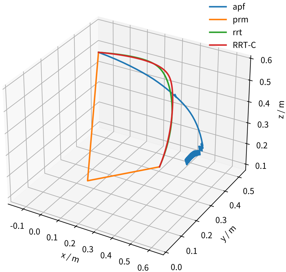
End-effector trajectory: scene_pass_through_maze
