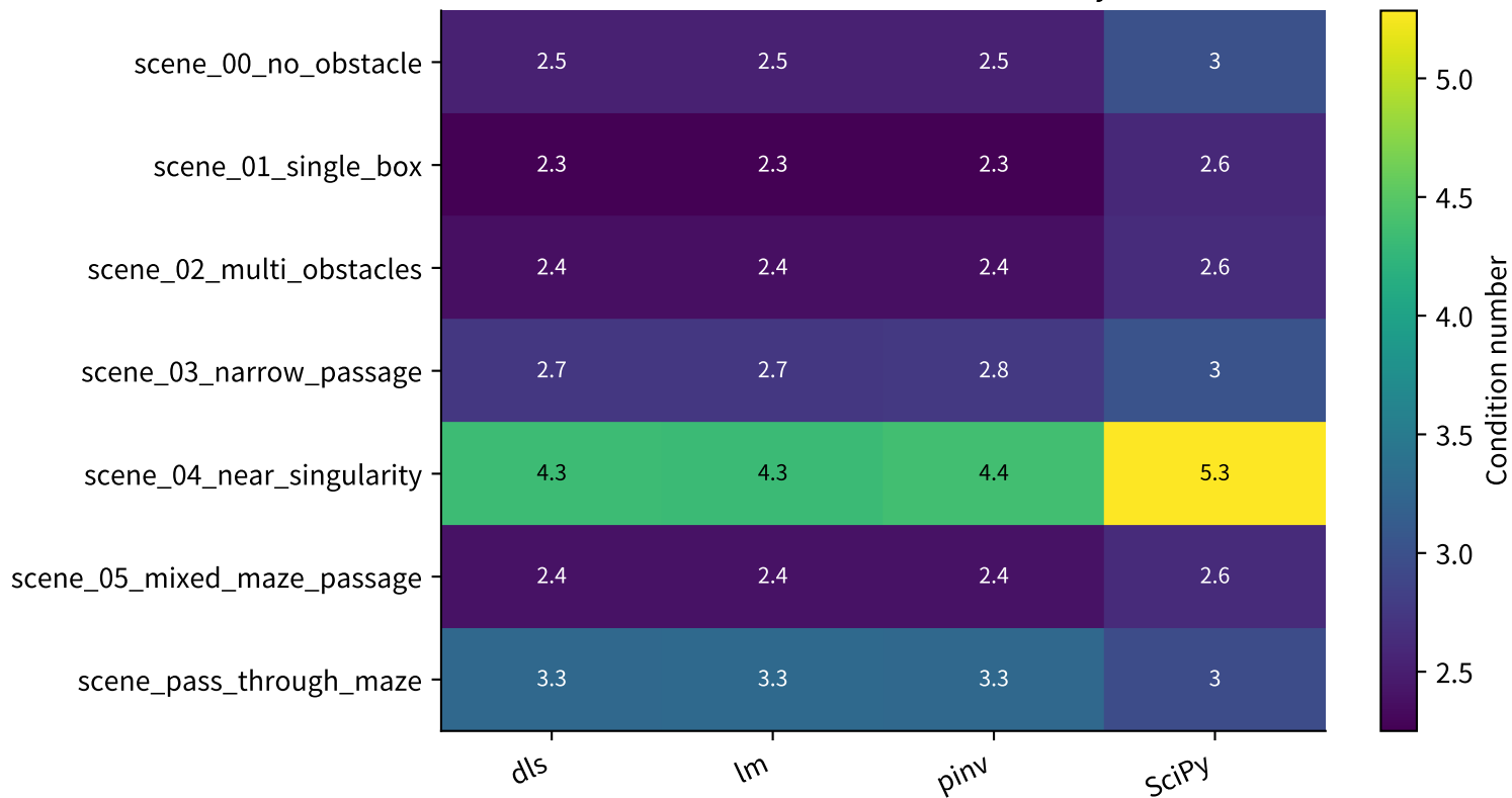
Mean Jacobian condition number by scene
