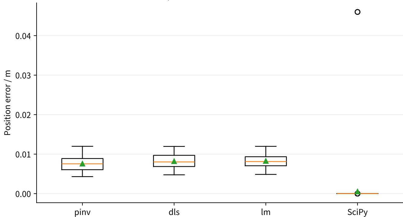
IK position error distribution
