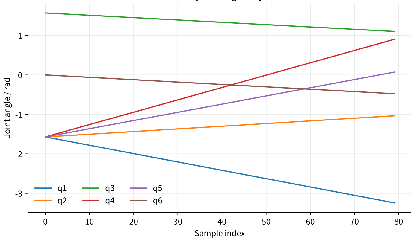
rrt_connect joint-angle trajectories
