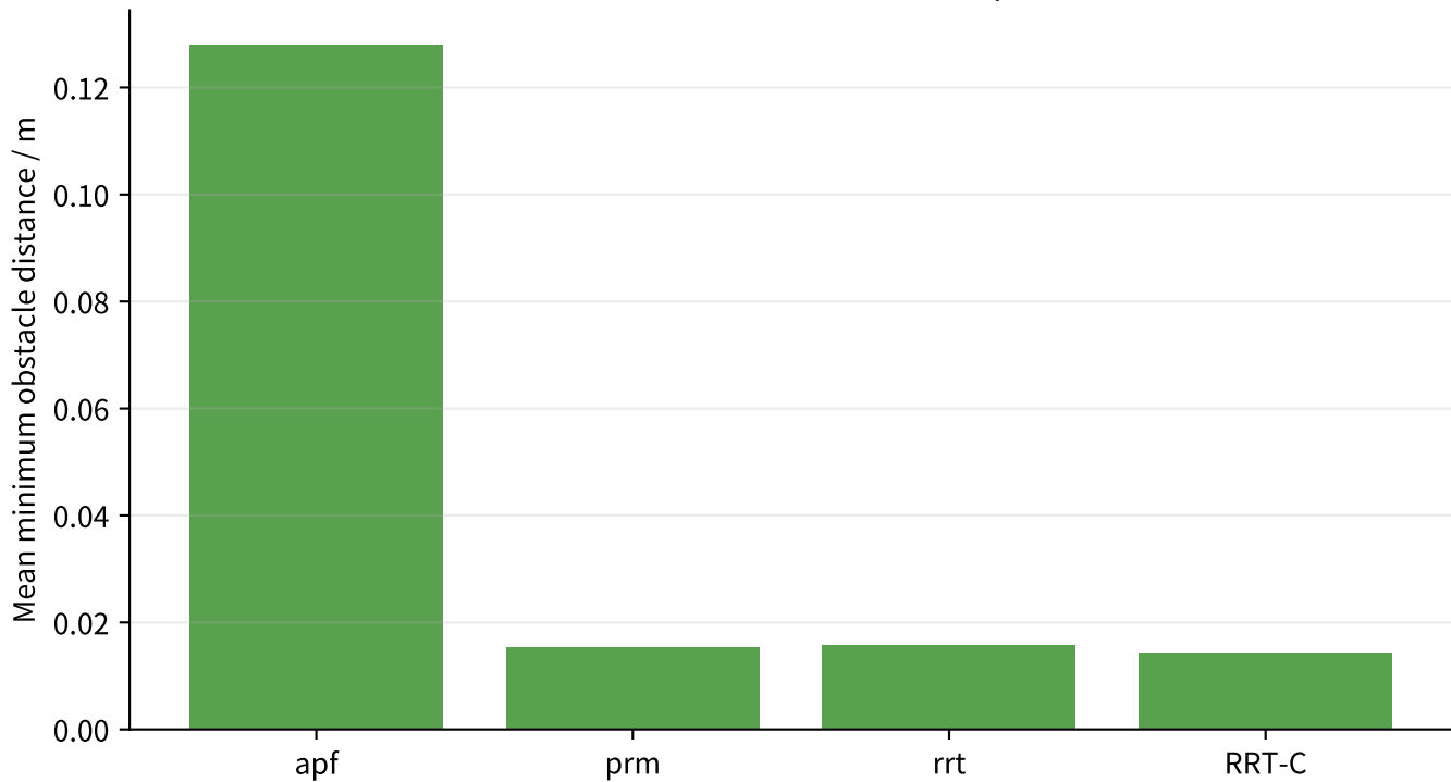
Minimum obstacle distance comparison
