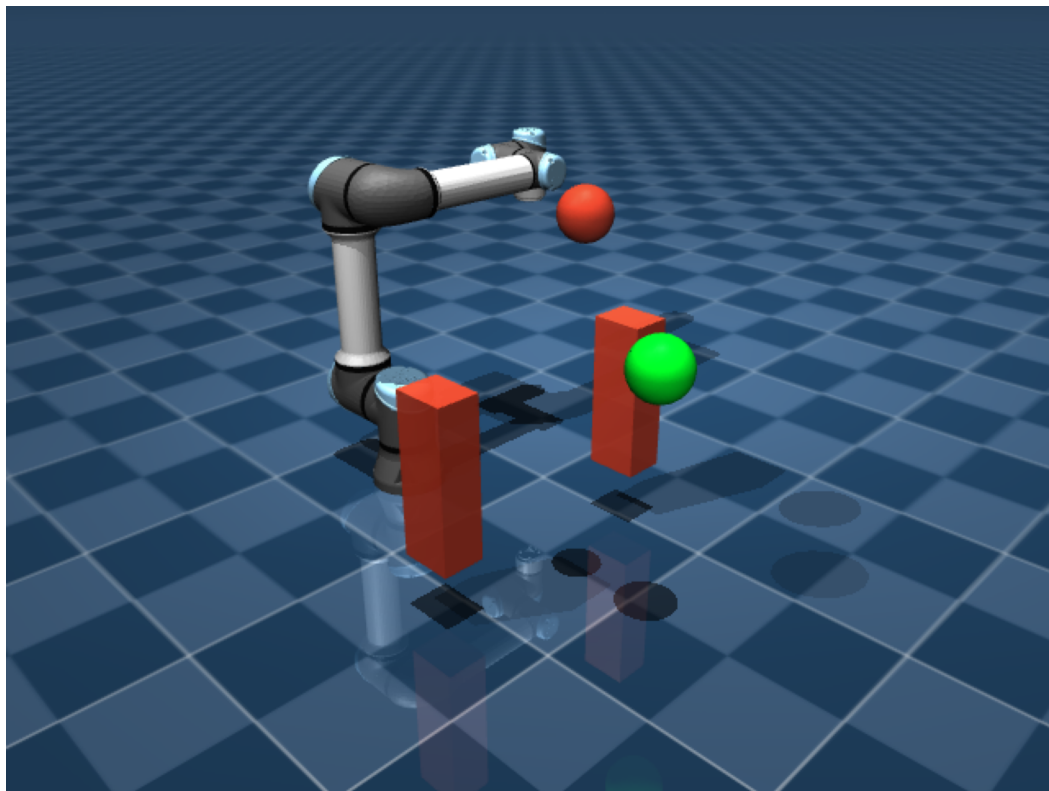
scene_03_narrow_passage
