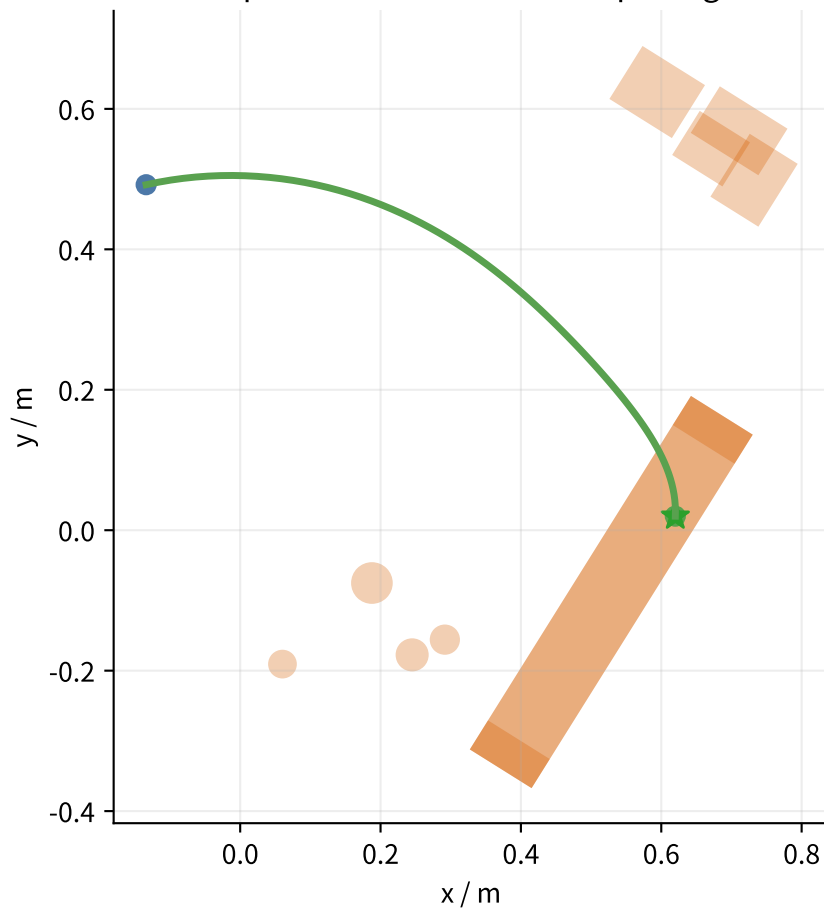
Top view of mixed obstacle passage
