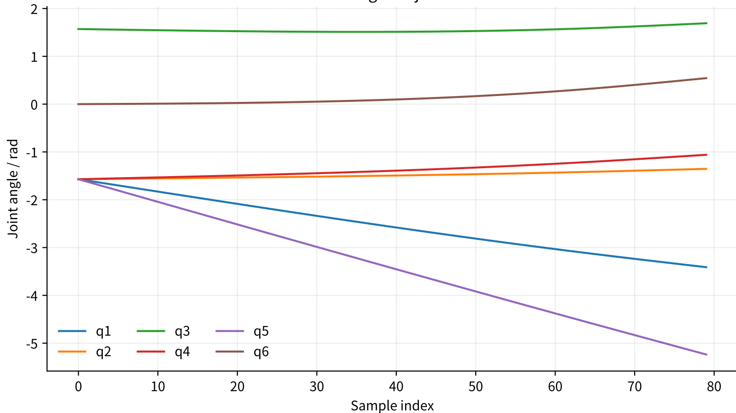
Joint-angle trajectories
