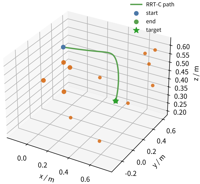
End-effector path through mixed maze
