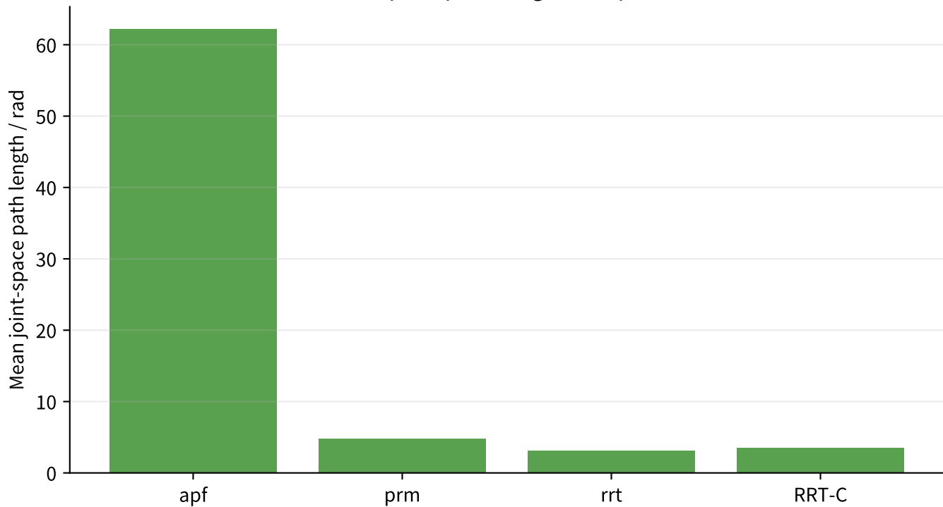
Joint-space path length comparison
