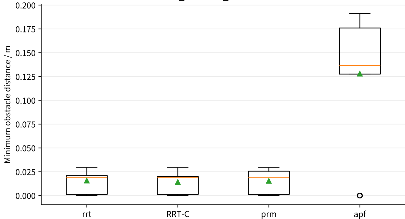
Planner min_obstacle_distance distribution
