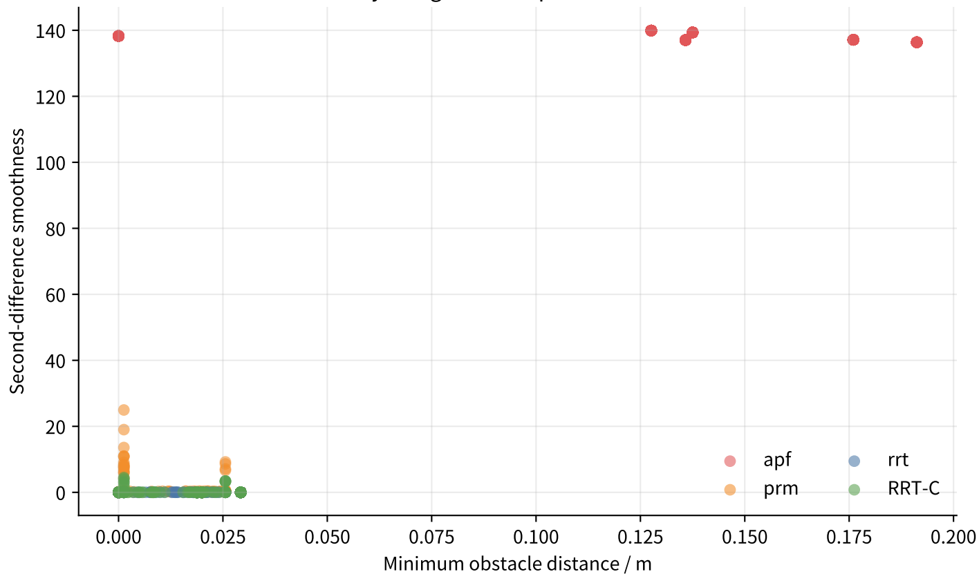
Safety margin versus path smoothness
