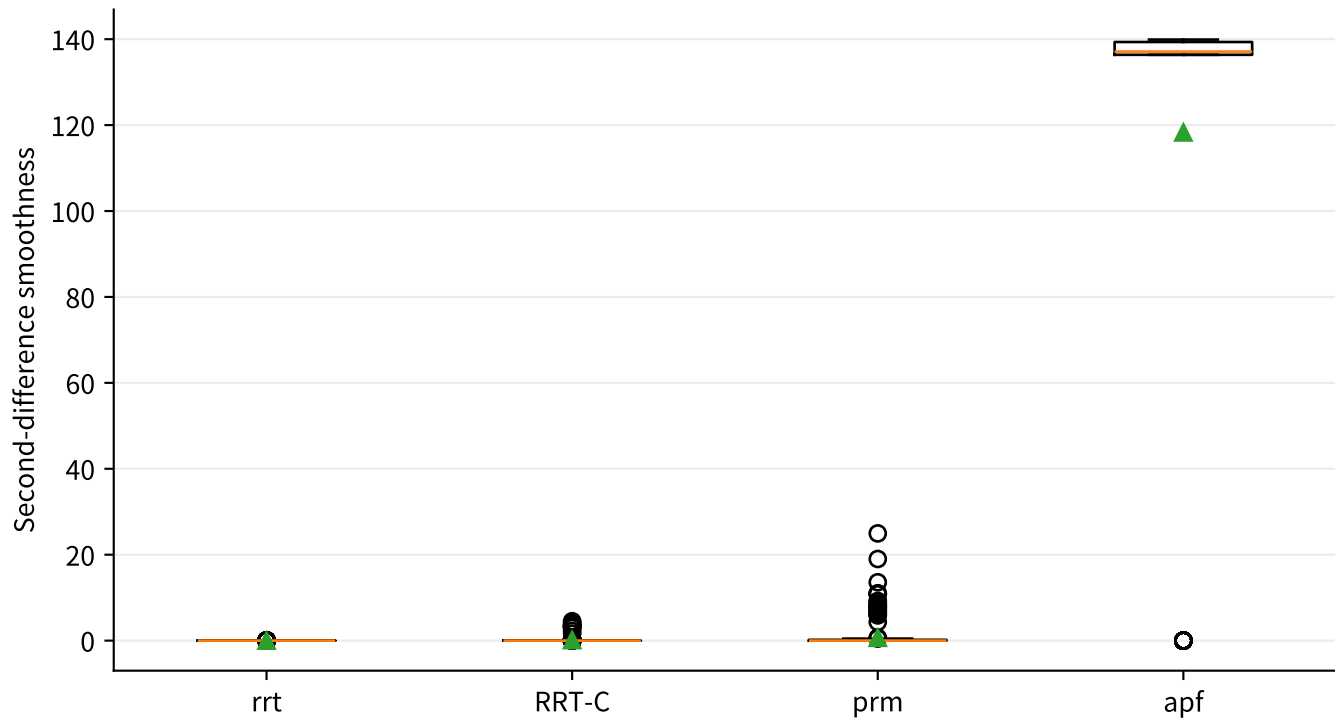
Planner smoothness distribution
