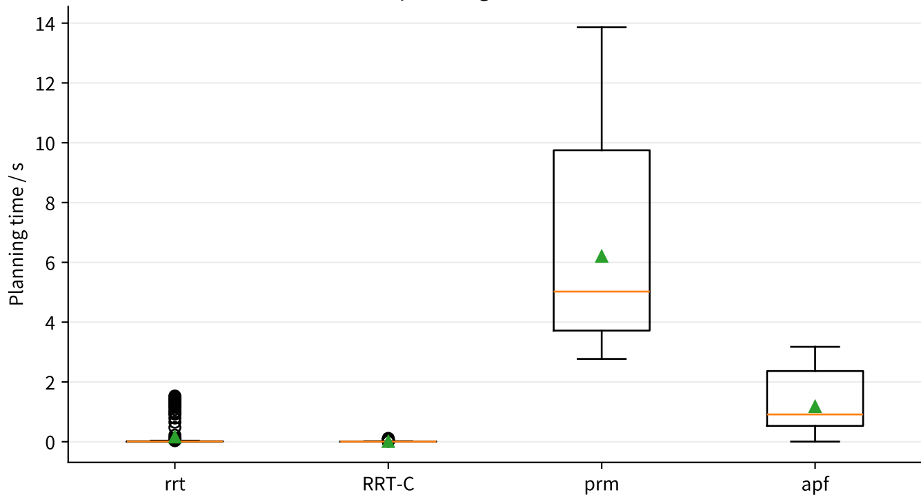
Planner planning_time distribution
