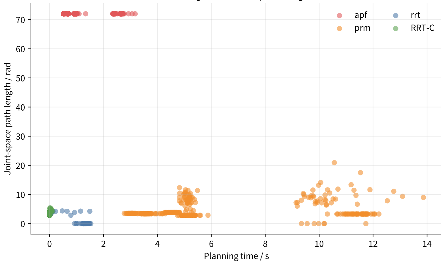
Planning time versus path length
