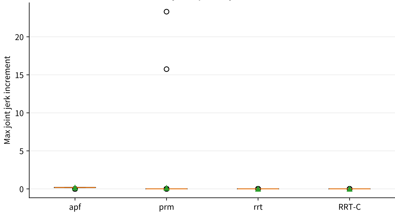
Derived trajectory max_jerk distribution
