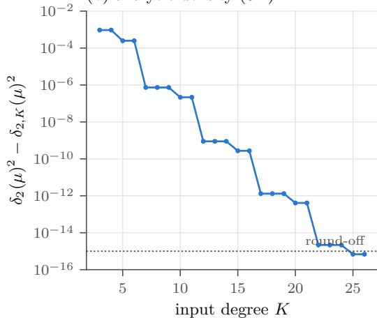
(b) analytic density (6.1)
