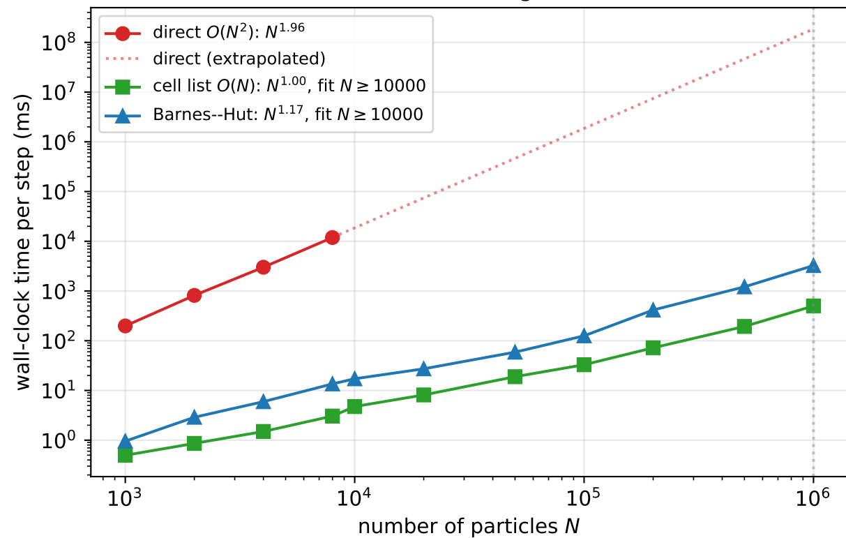
(a) Wall-clock scaling to N = 10^6
