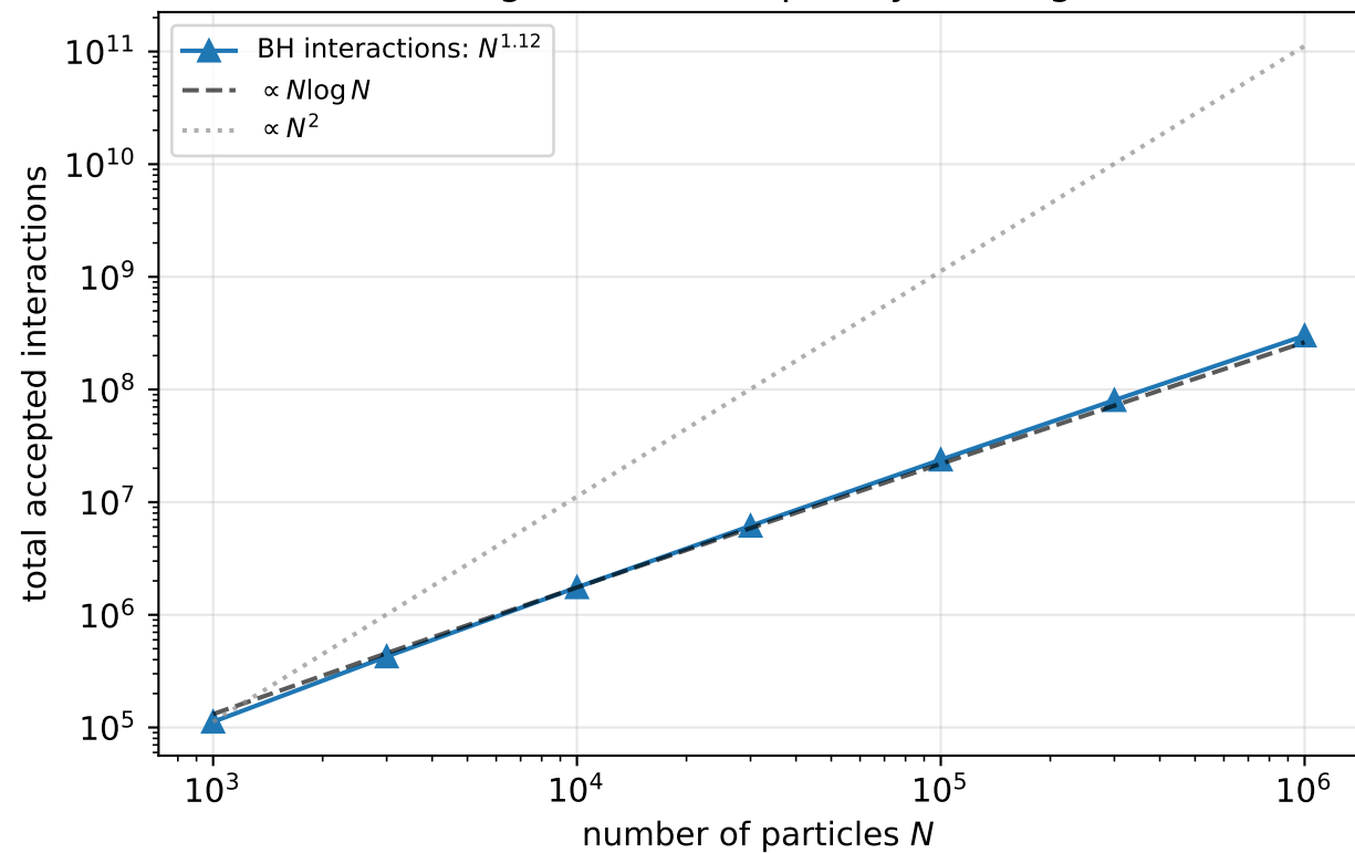
(b) Algorithmic complexity: O(N \log N)
