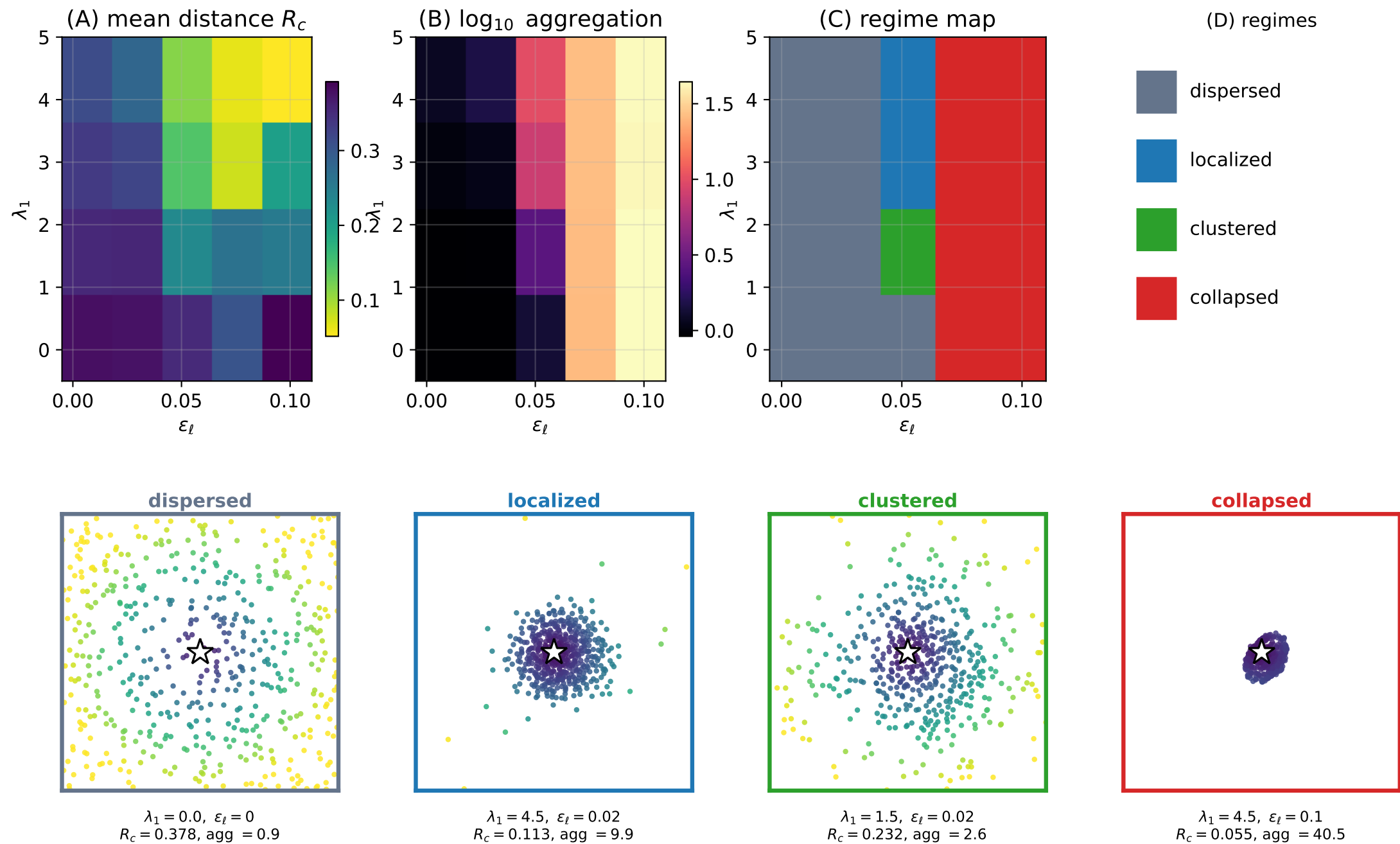
Figure 2. Emergent macroscopic regimes over the (\lambda_1, \varepsilon_\ell) parameter space
