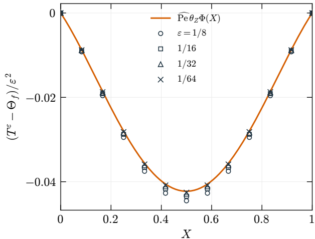
(b) Cross-channel variation at y = \frac{1}{2}
