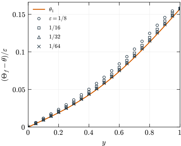
(a) Scaled leading fin error
