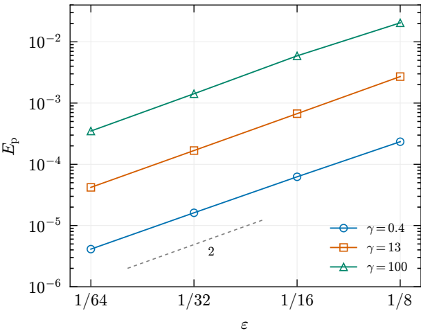
(a) Corrected fluid error
