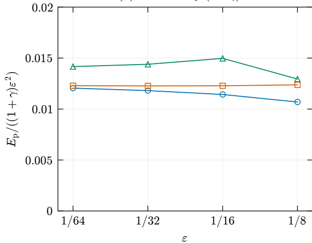
(b) Rescaled by (1 + \gamma)\varepsilon^2
