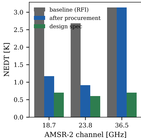
(b) radiometric noise restored
