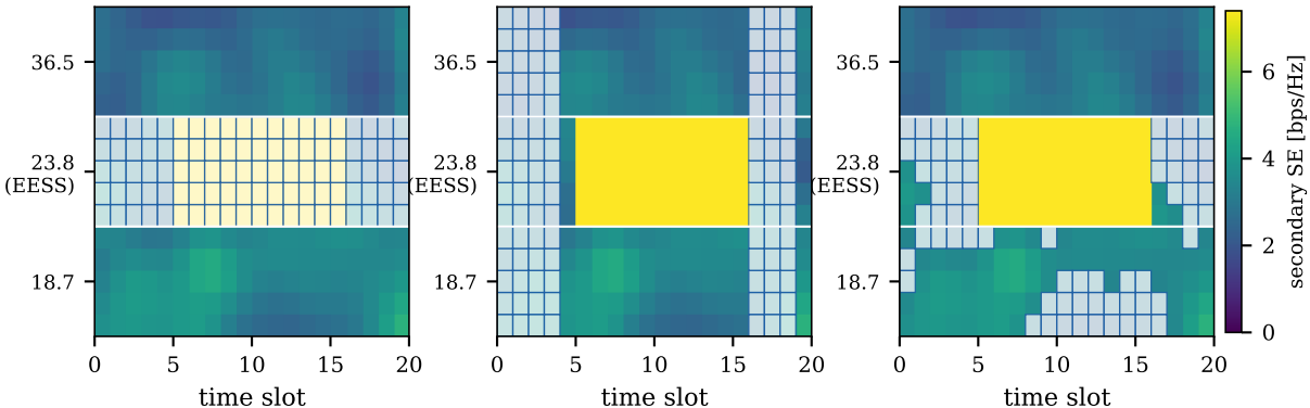
(a) static partitioning (100 tiles, TPW 1.39\,mm: infeasible) (b) best fixed-window muting (105 tiles, TPW 0.97\,mm, 4.06\,Gb/s) (c) proposed procurement (69 tiles, TPW 1.00\,mm, 4.97\,Gb/s)
