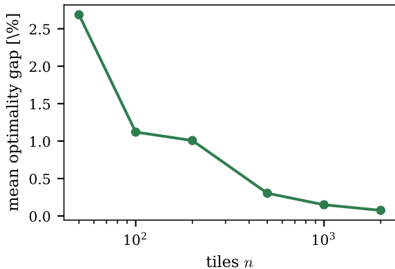
(b) gap vs. exact DP (20 seeds/point)
